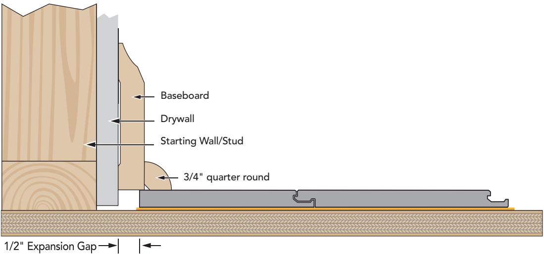
TYPICAL INSTALLATION
